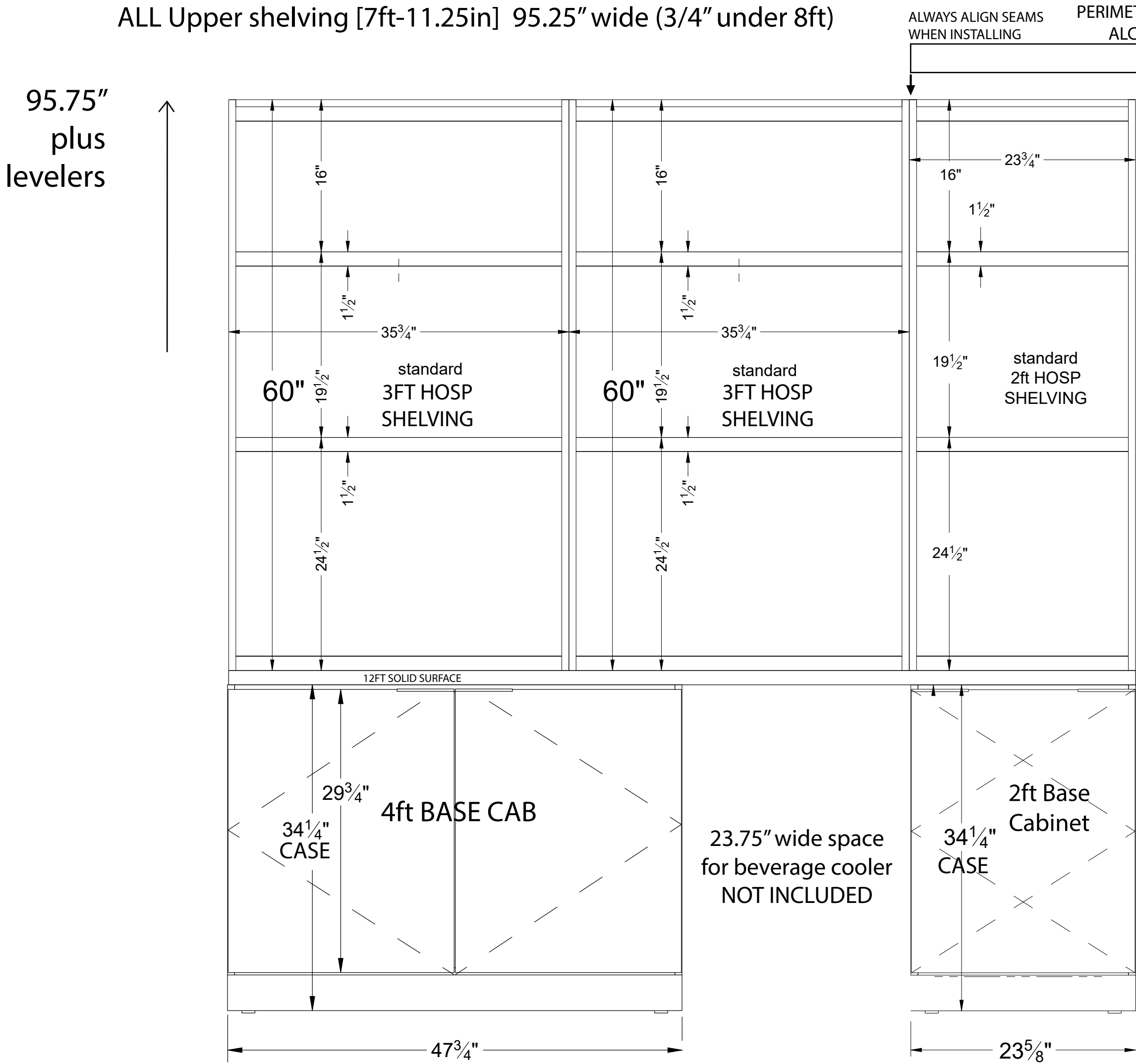
FRONT VIEW
